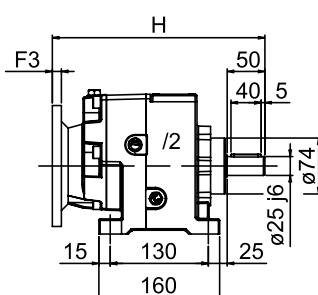
Modular Flange Brida modular
